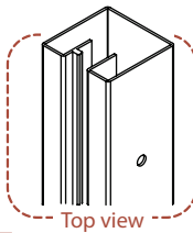
Right Post (2) 1 1/8" x 1 1/8" x 48"
